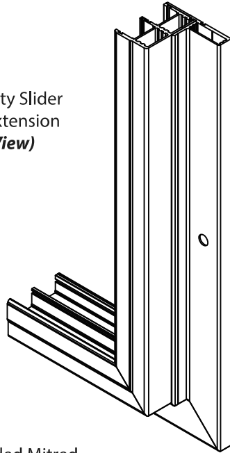
4-Sided Mitred Extension Shown
