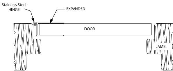
Hinge Expander Installation
