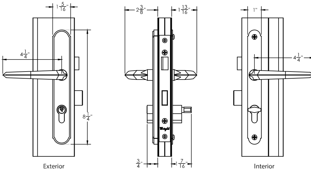
* C5374BL Tru-Frame® and TruView™ Hardware Dimensions
