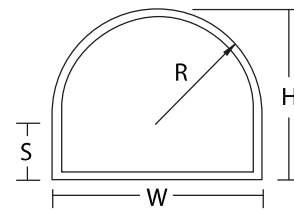
HALF CIRCLE W/ EXTENDED LEGS
